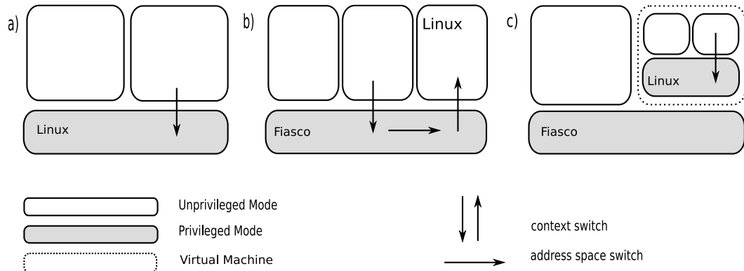
Figure 4.1: System call execution in (a) native Linux, (b) L4Linux and (c) Linux in a VM.
