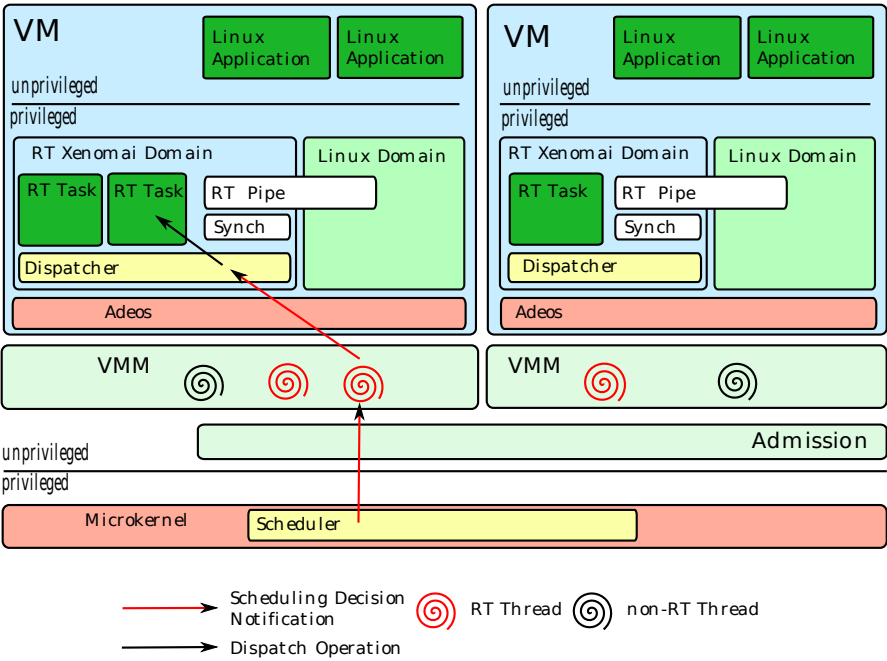
Figure 7.3: Real-time VM setup
