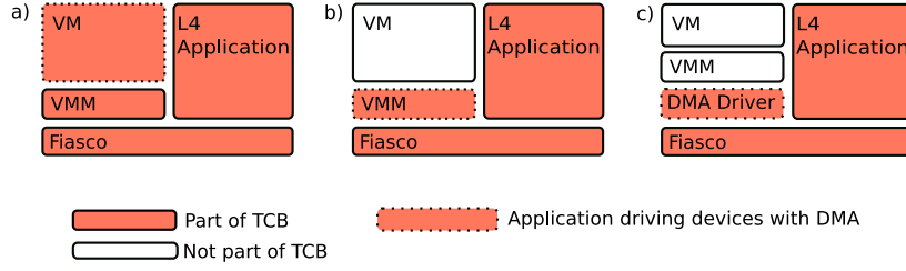
Figure 4.4: TCB of an L4 application where (a) the VM drives the hard disk, (b) hard disk commands are mediated by the VMM and (c) hard disk commands are handed out to an external server.
