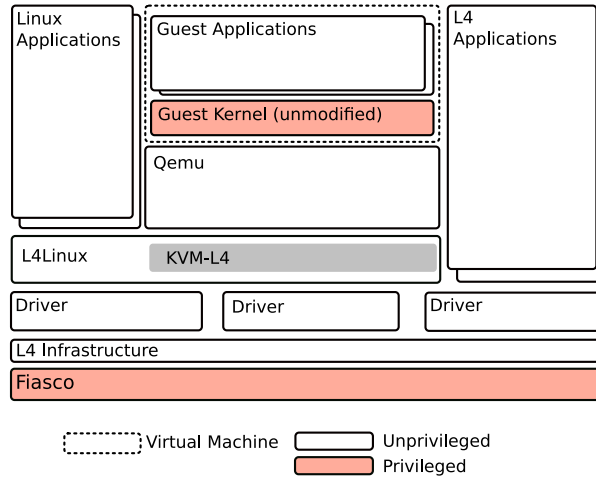
Figure 3.7: KVM-L4 running one VM and L4 applications with a small trusted computing base side-by-side.
