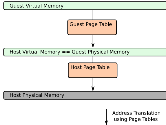
Figure 2.2: MMU virtualization without VMM intervention: Nested paging.
