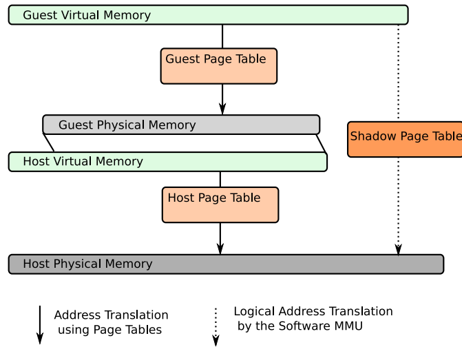
Figure 2.1: Illustration of a shadow page table that maps guest virtual to host physical addresses.
