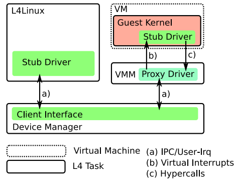
Figure 5.3: On the left hand side there is a standard L4Linux kernel with a stub driver. The stub driver consists of the driver logic and the L4 IPC interface for communication with the L4 device manager. On the right hand side both Karma and a Linux VM are depicted. The stub driver in the Linux kernel has been split so that the driver logic remains inside of Linux, and the L4 IPC interface resides in the VMM. A custom hypercall-based protocol connects both parts.
