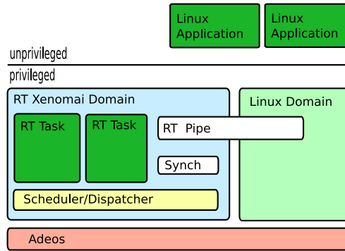
Figure 7.1: Xenomai architecture
