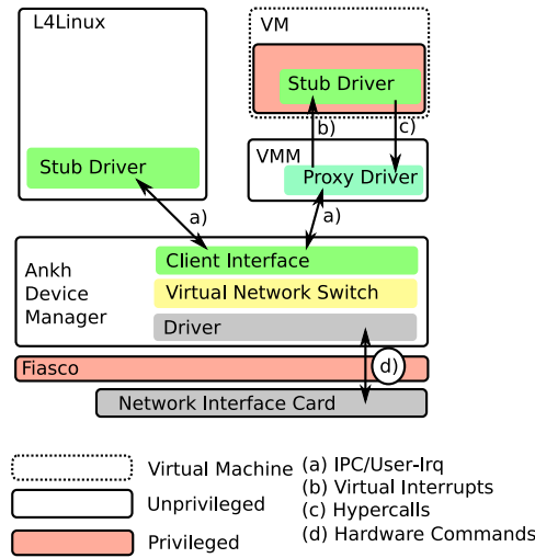
Figure 5.4: The Ankh network multiplexer with two clients: L4Linux and a VM running Linux.
