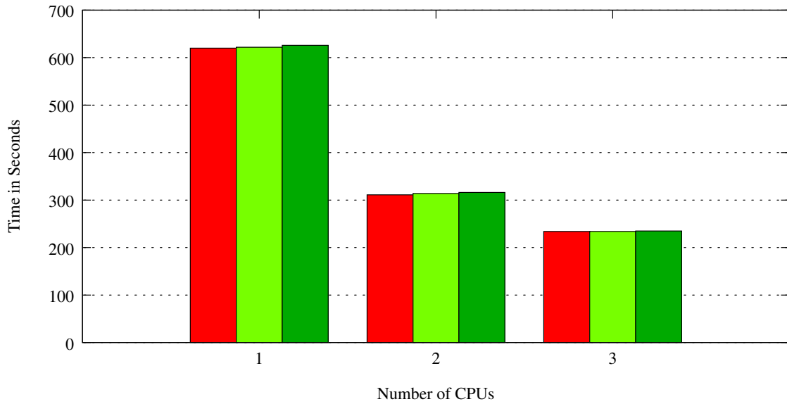
Figure 6.12: Kernel compile benchmarks with a custom slowdown of the world switch path. The red bars denote zero slowdown, light green denotes a slowdown of 5000 CPU cycles and the dark green bar denotes a slowdown of 10000 CPU cycles.
