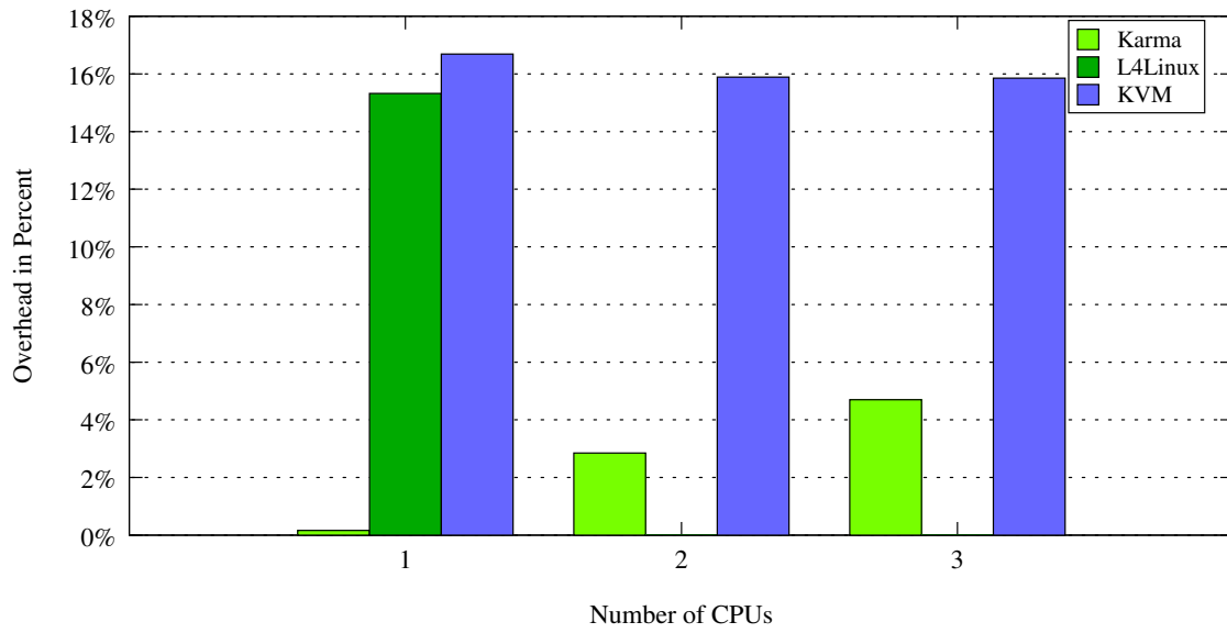
Figure 6.7: Kernel compile overhead relative to native Linux. No data is available for L4Linux on 2 and 3 processor setups.
