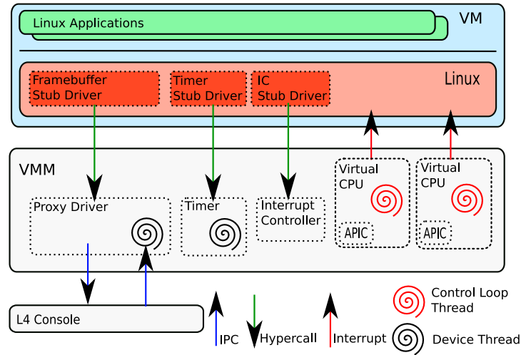
Figure 4.6: Envisioned system architecture.
