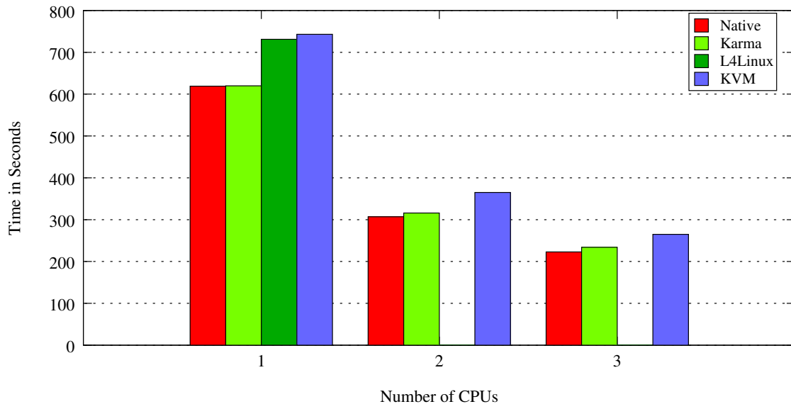
Figure 6.6: Kernel compile times
