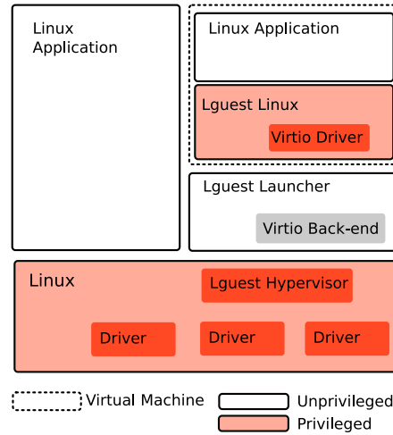
Figure 3.4: Linux running a para-virtualized Linux in a VM using the Lguest hypervisor.
