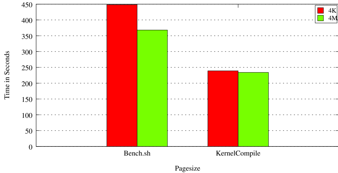
Figure 6.11: Comparison Performance of Bench.sh and a kernel compilation with 4K and with 4M pages (superpages).
