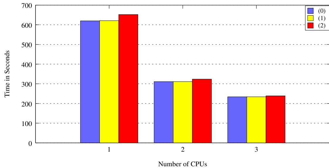
Figure 6.10: Comparison of kernel compile different types of direct hard disk access. (0) is the kernel compile in VM with direct hard disk access, whereas in (1) and (2), Linux has no access to IO memory and instructs Karma via hypercalls. In (1) Karma spends 10000 cycles before writing the command and 3000 cycles before reading values, to simulate analysis of the commands. In (2) Karma waits 100000 cycles before writing and 30000 before read, to simulate command analysis by a separate task.
