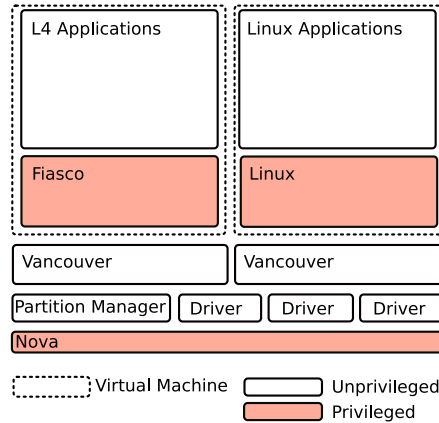
Figure 3.5: NOVA OS Virtualization Architecture, running a VM with Linux and one with Fiasco.
