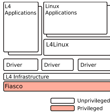
Figure 3.1: L4Linux running as a user land server on top of the L4 microkernel Fiasco.
