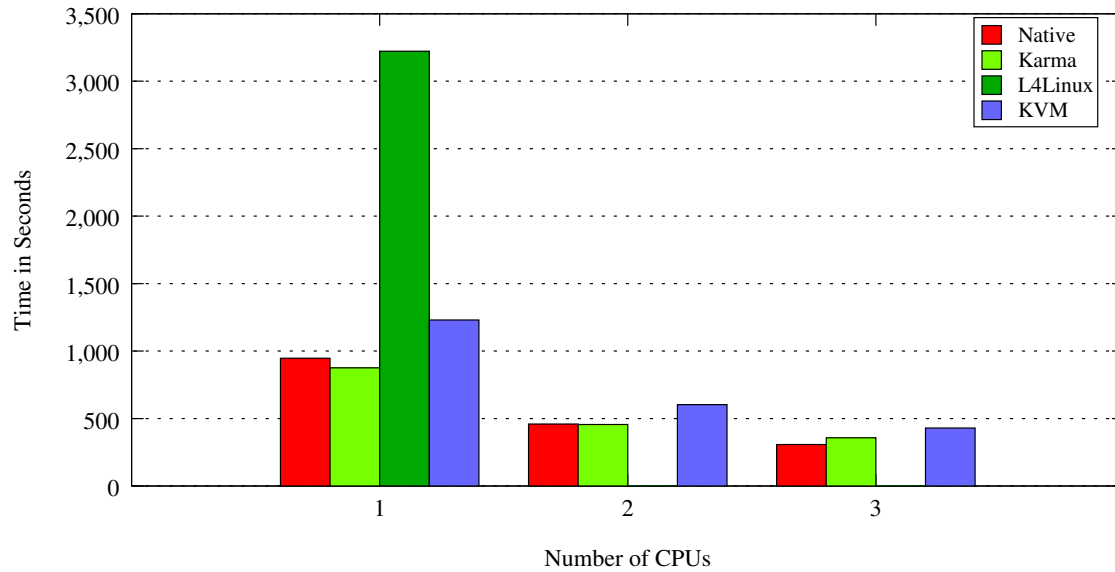
Figure 6.4: Bench.sh benchmark
