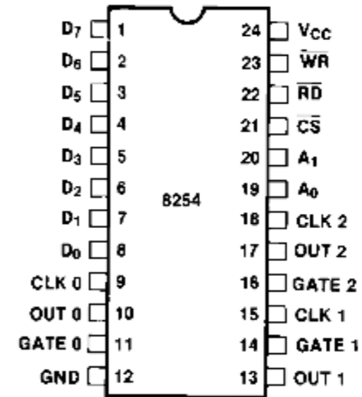
Figure 2. Pin Configuration
